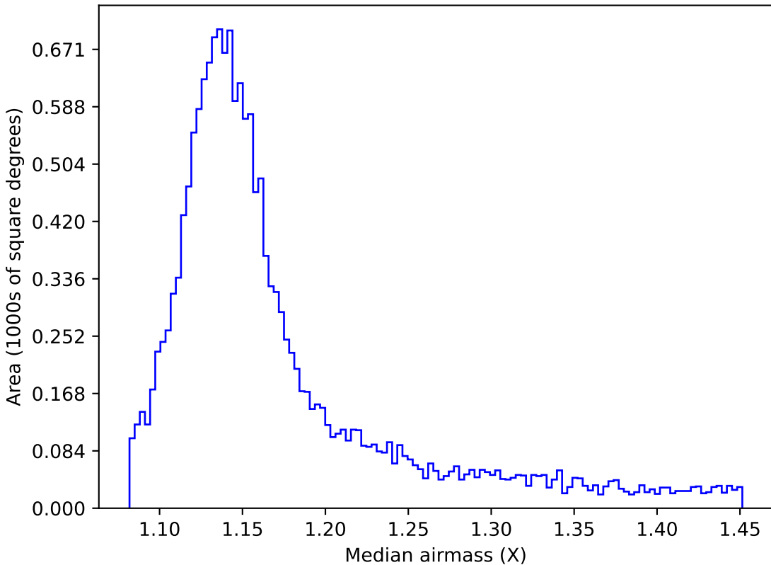
baseline_v2.0_10yrs WFD z band: Median airmass
