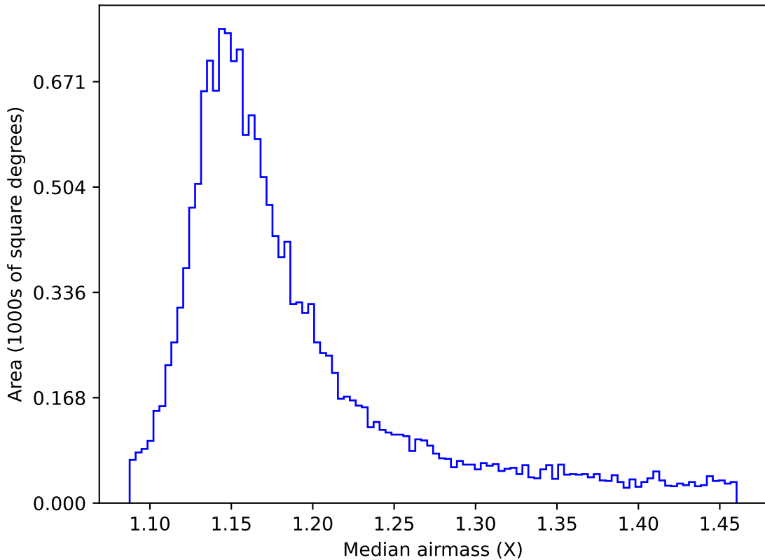
baseline_v2.0_10yrs WFD y band: Median airmass
