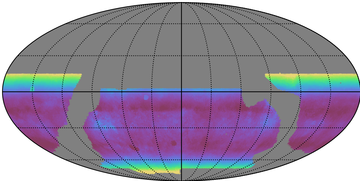
baseline_v2.0_10yrs WFD r band: Median airmass
