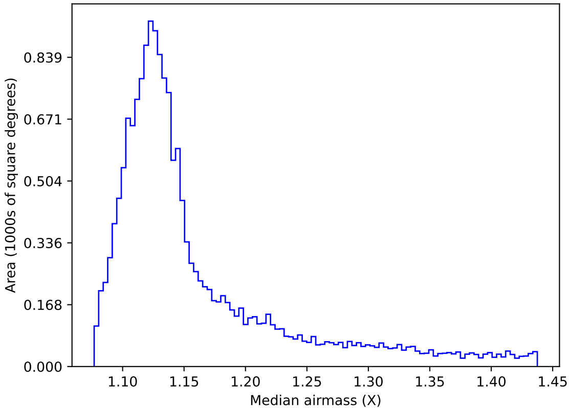
baseline_v2.0_10yrs WFD r band: Median airmass
