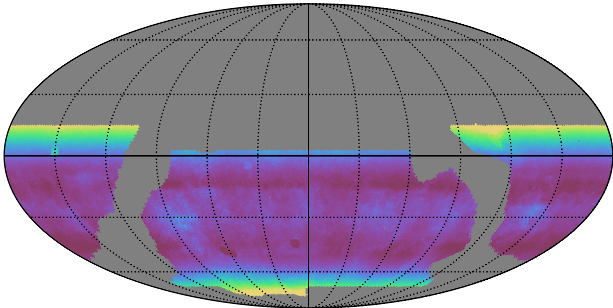
baseline_v2.0_10yrs WFD i band: Median airmass
