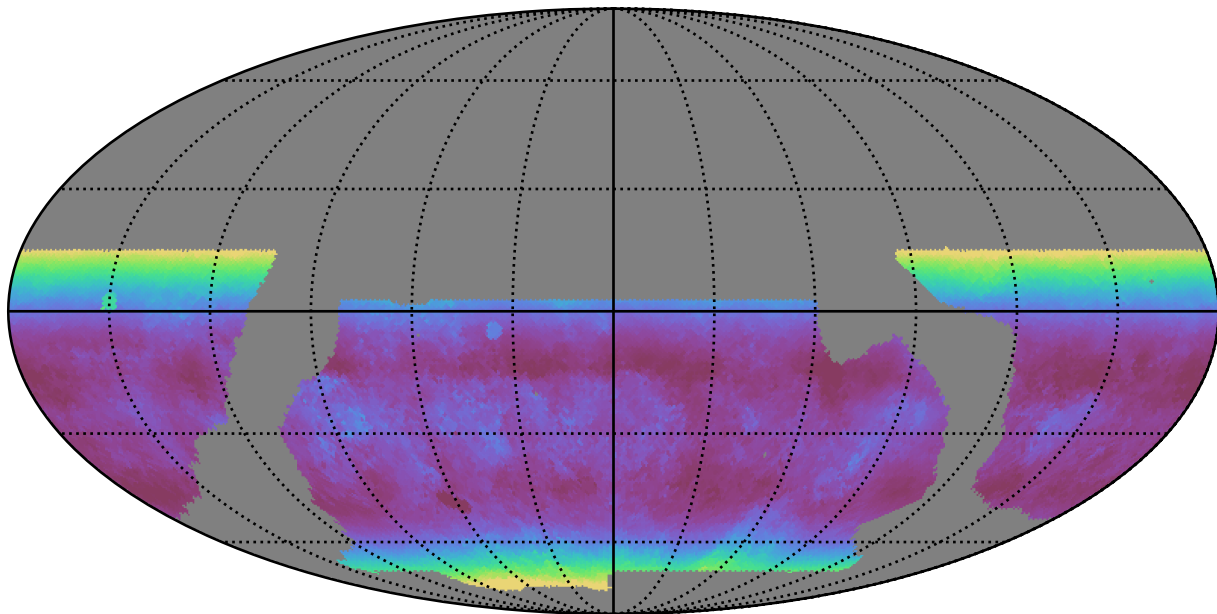
baseline_v2.0_10yrs WFD g band: Median airmass
