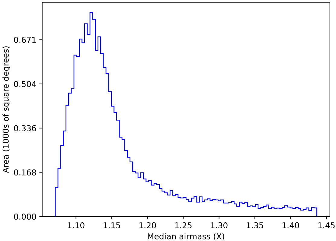
baseline_v2.0_10yrs WFD g band: Median airmass
