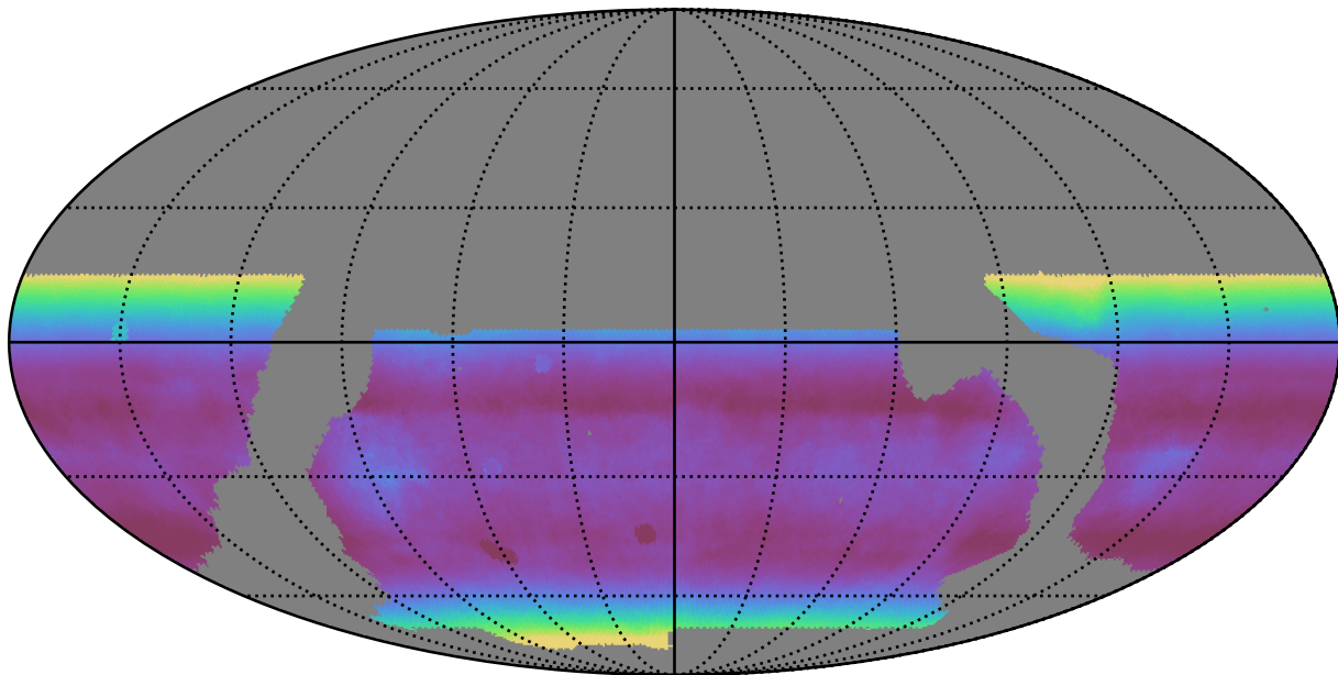
baseline_v2.0_10yrs WFD all bands: Median airmass
