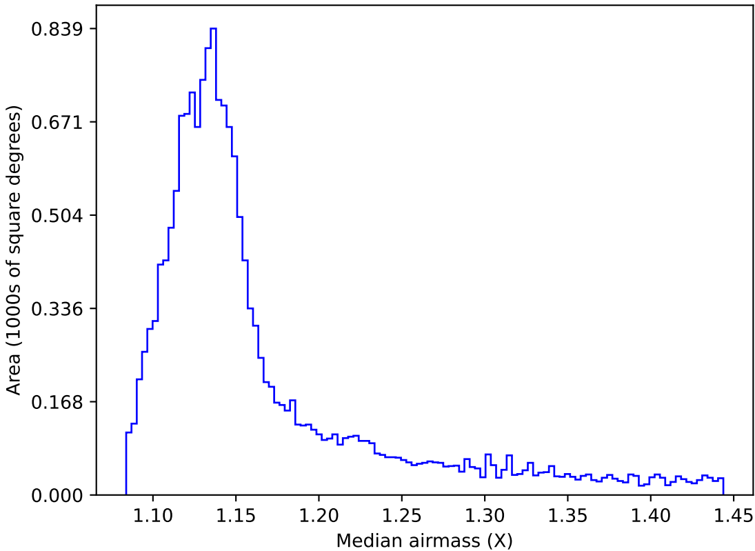
baseline_v2.0_10yrs WFD all bands: Median airmass
