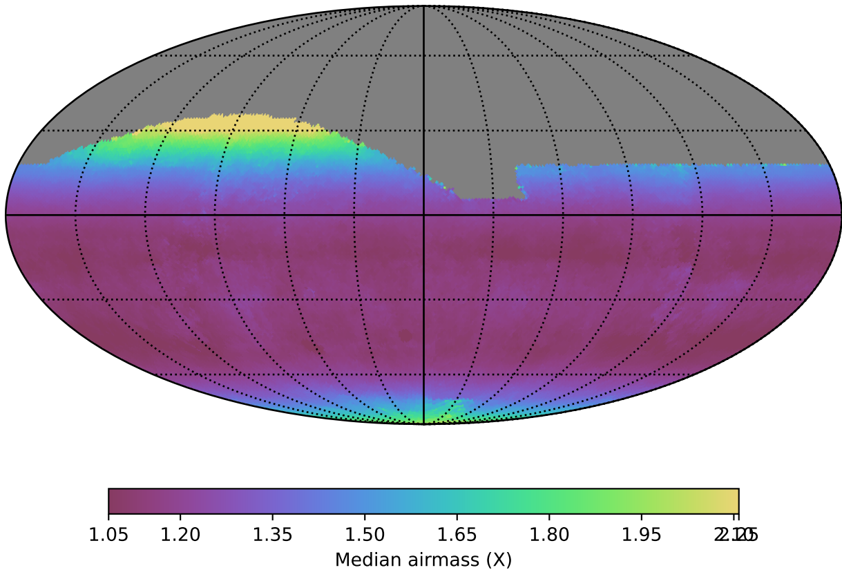
baseline_v2.0_10yrs All sky z band: Median airmass
