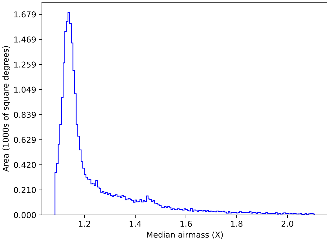
baseline_v2.0_10yrs All sky z band: Median airmass
