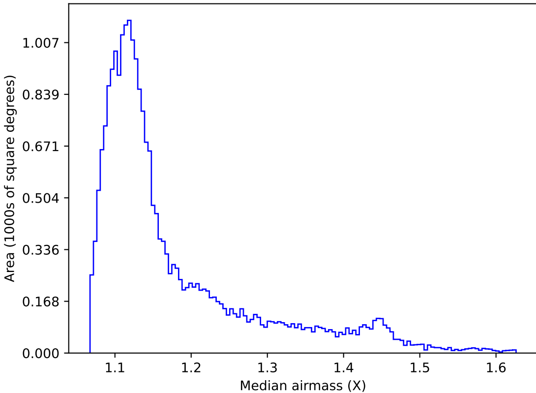
baseline_v2.0_10yrs All sky u band: Median airmass
