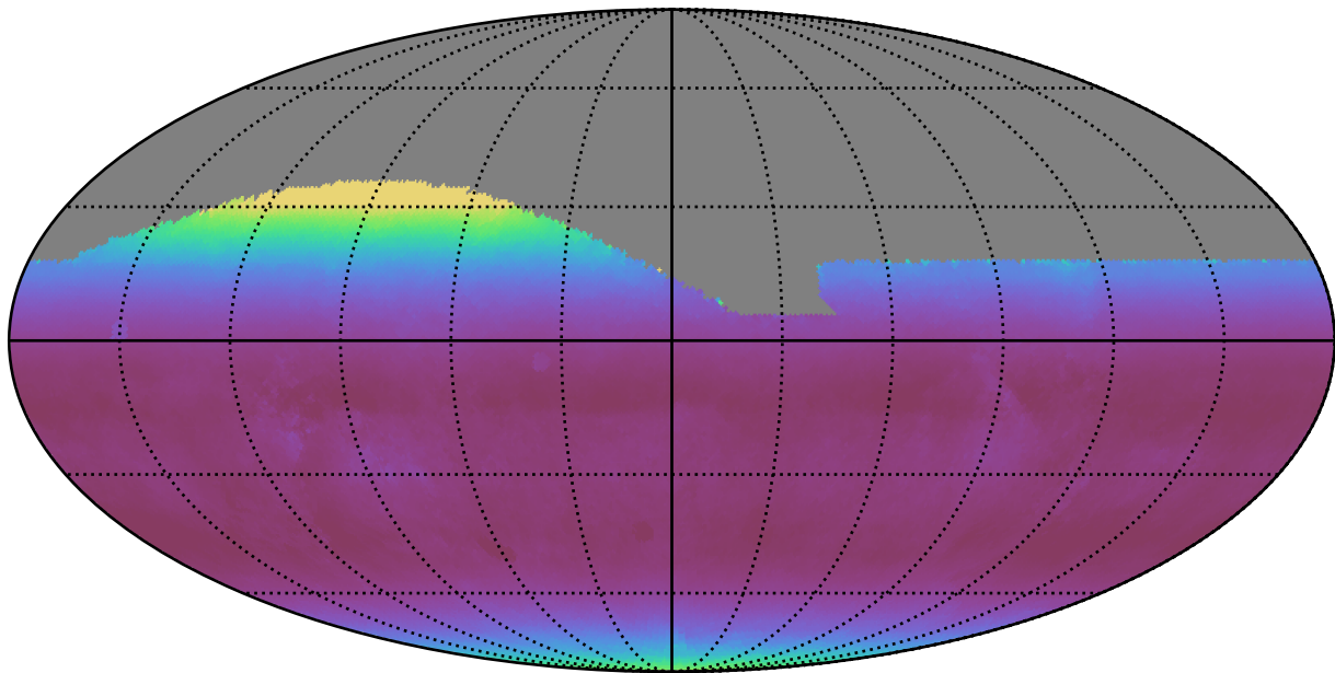
baseline_v2.0_10yrs All sky r band: Median airmass
