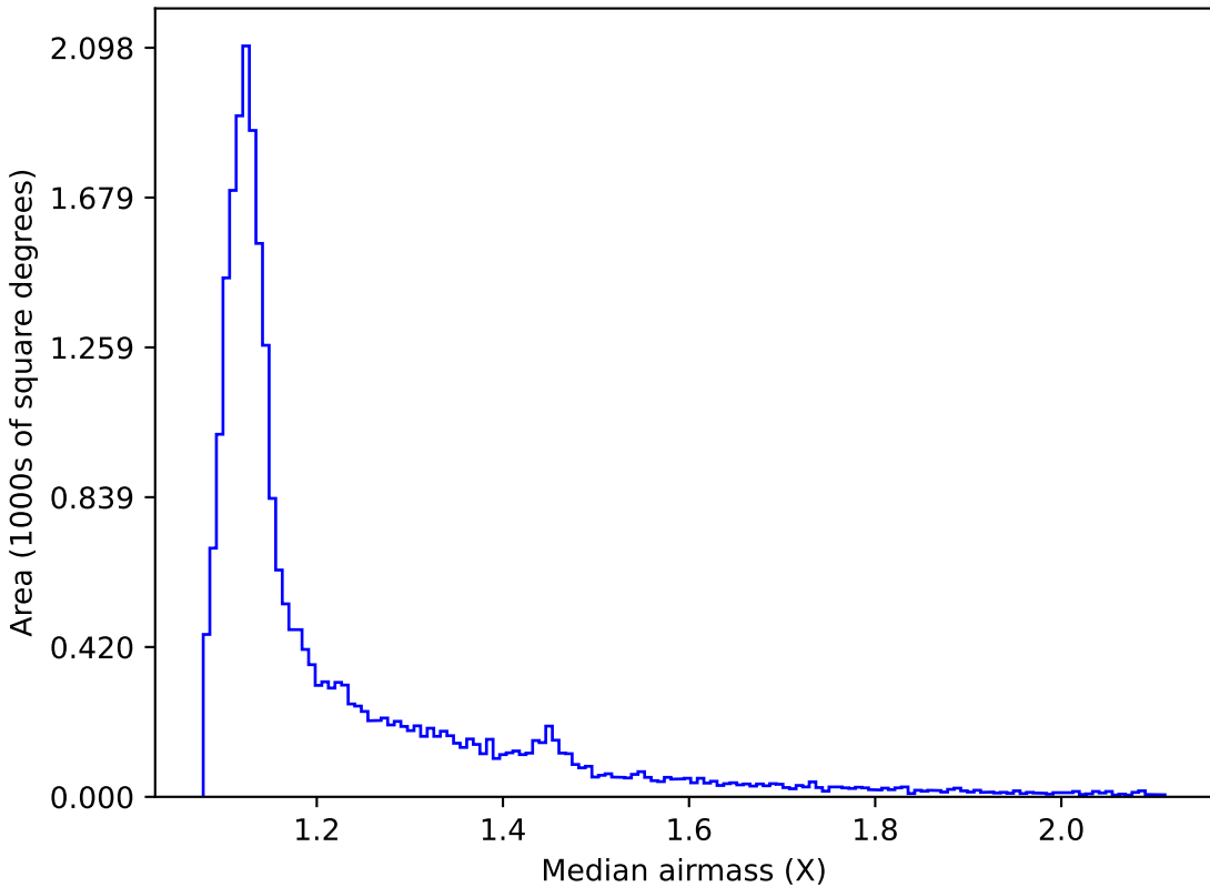
baseline_v2.0_10yrs All sky r band: Median airmass
