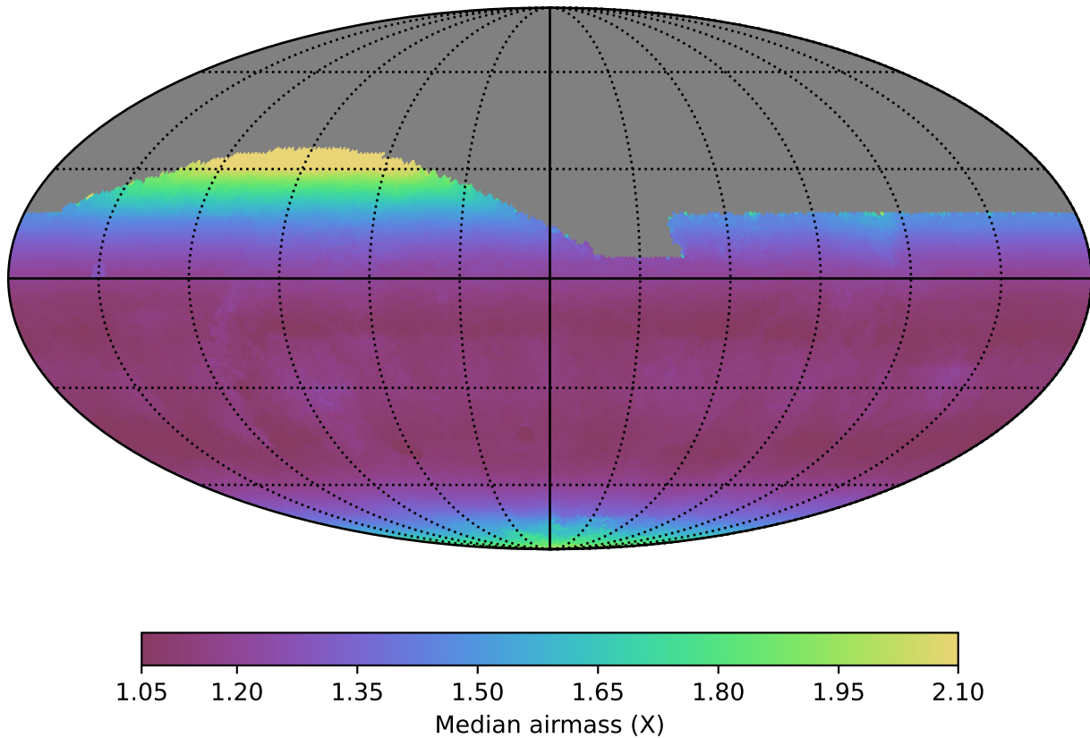
baseline_v2.0_10yrs All sky i band: Median airmass
