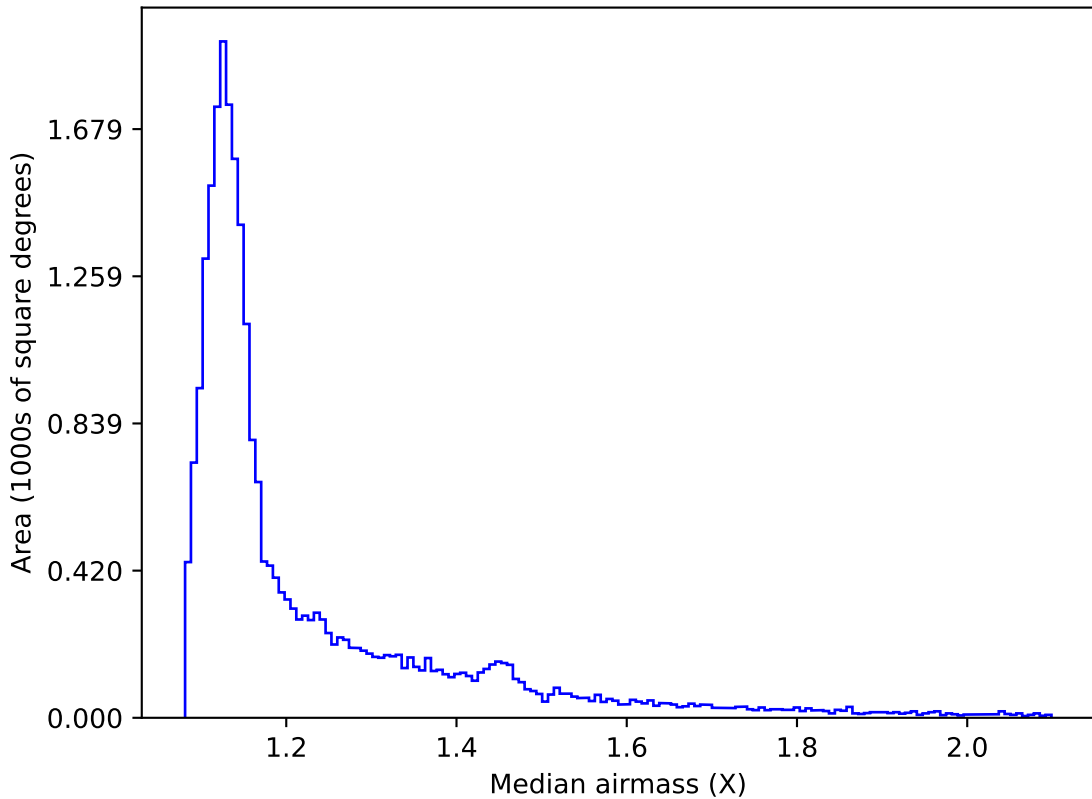
baseline_v2.0_10yrs All sky i band: Median airmass
