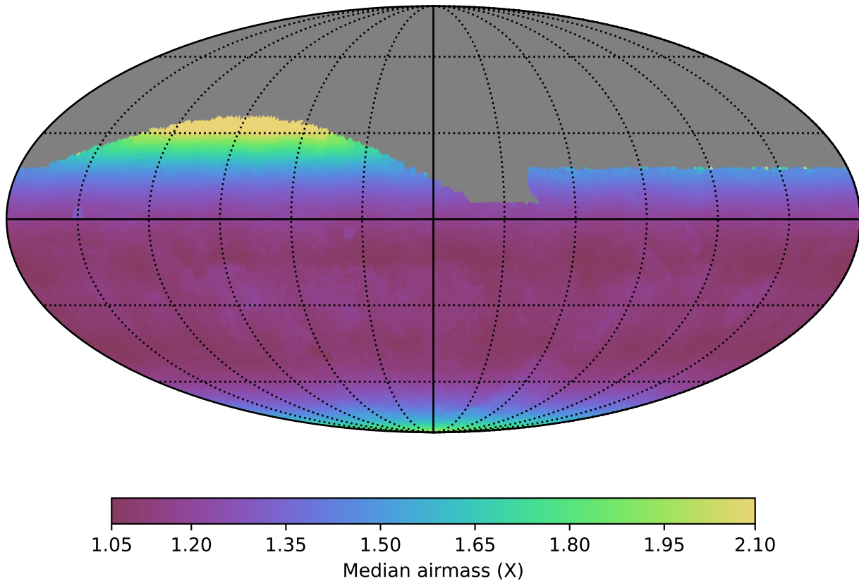
baseline_v2.0_10yrs All sky g band: Median airmass
