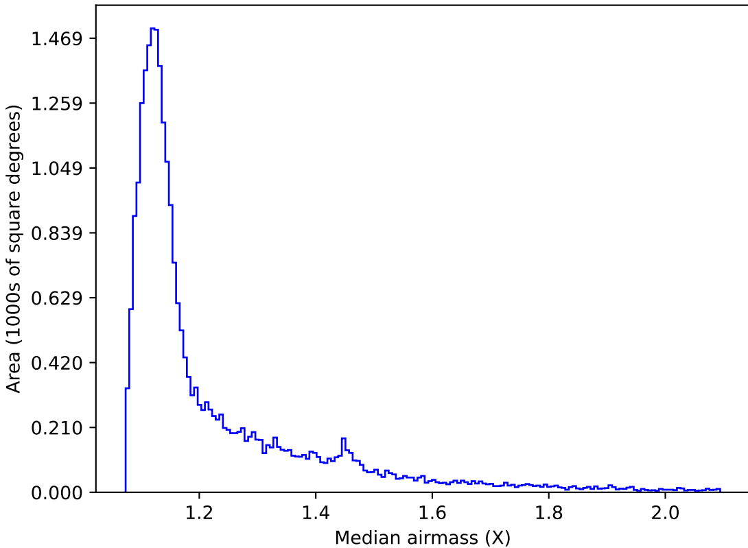
baseline_v2.0_10yrs All sky g band: Median airmass
