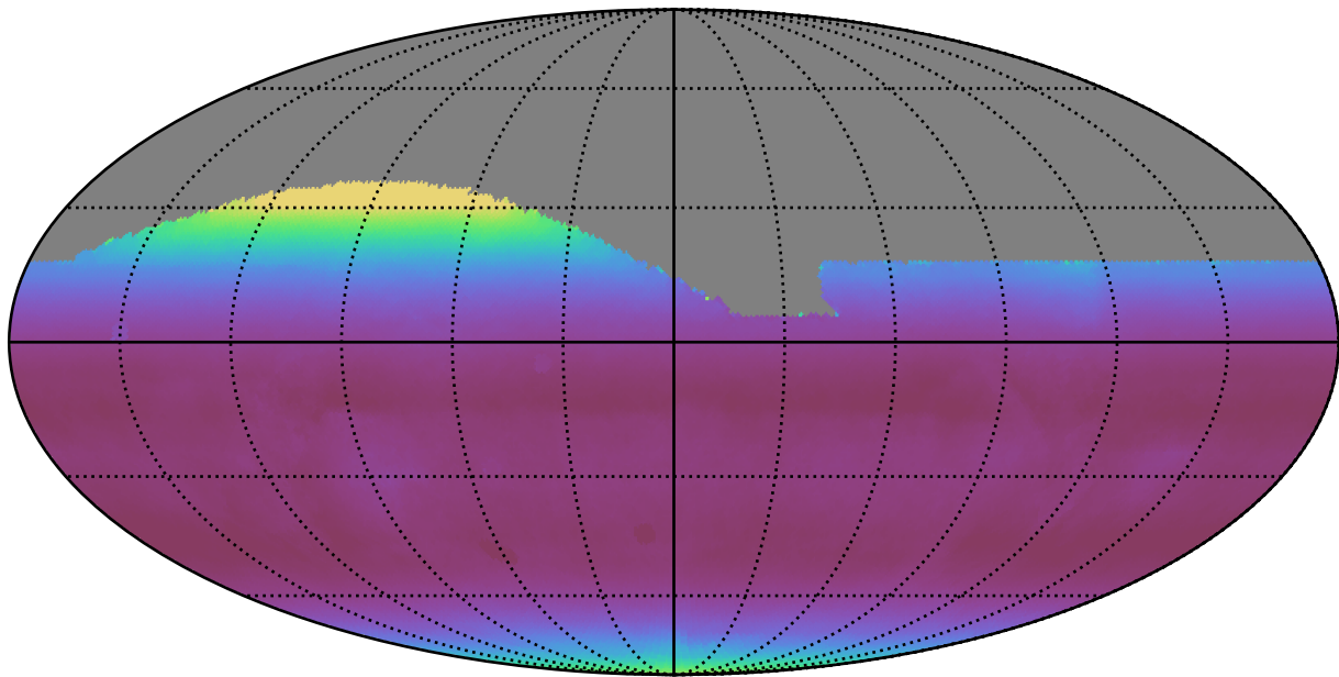
baseline_v2.0_10yrs All sky all bands: Median airmass
