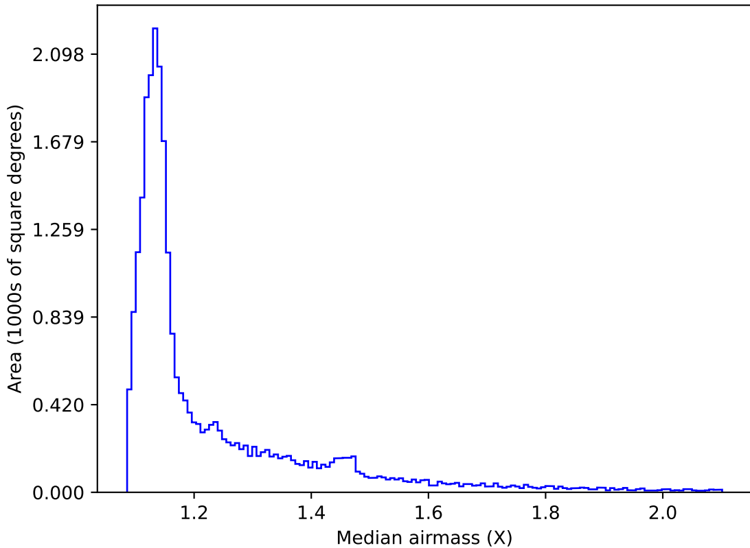
baseline_v2.0_10yrs All sky all bands: Median airmass
