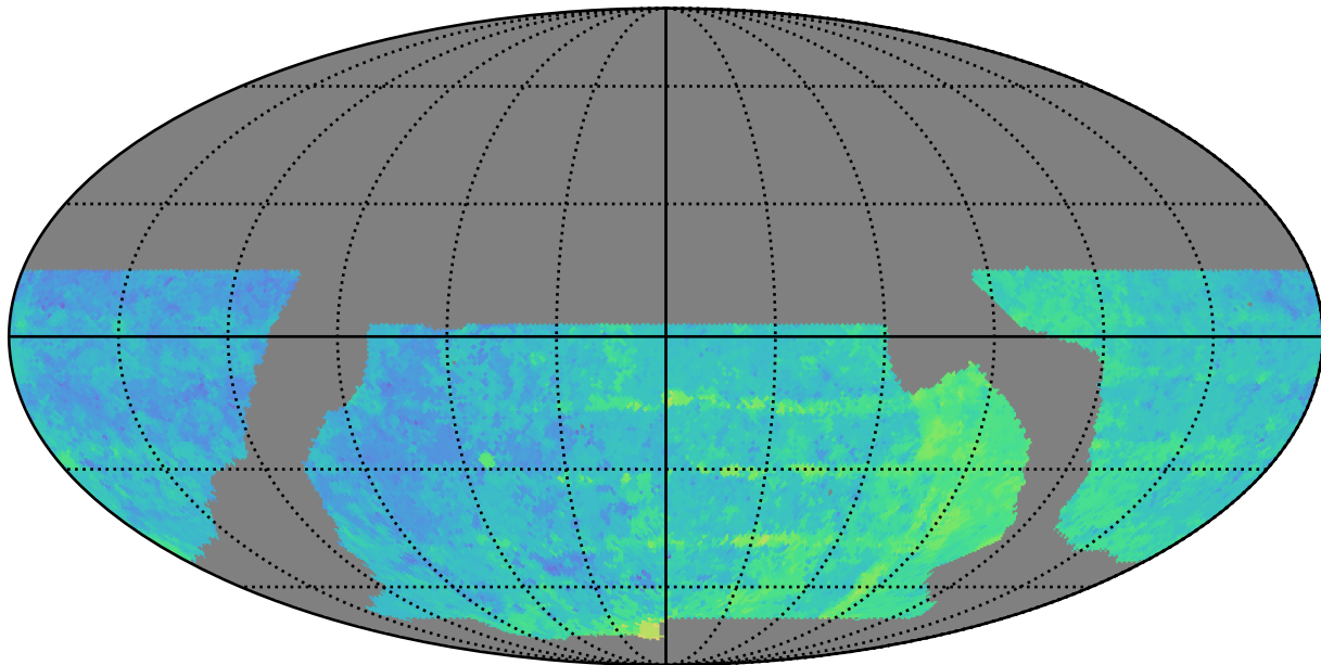
baseline_v2.0_10yrs WFD z band: Median Season Length
