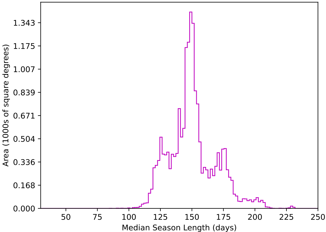
baseline_v2.0_10yrs WFD z band: Median Season Length
