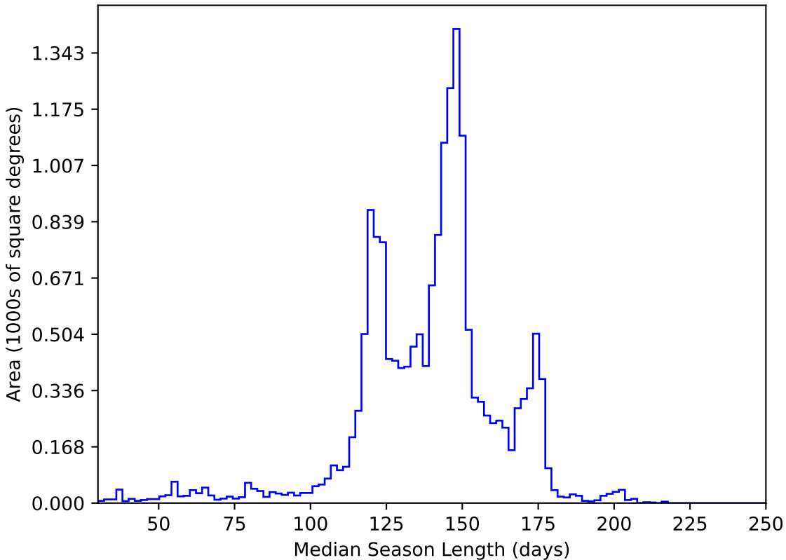
baseline_v2.0_10yrs WFD y band: Median Season Length
