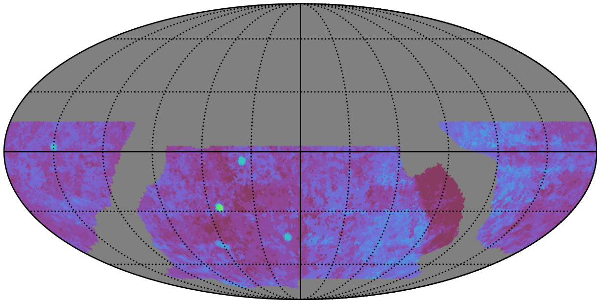
baseline_v2.0_10yrs WFD u band: Median Season Length
