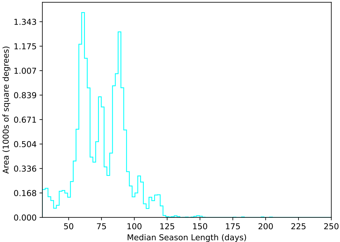
baseline_v2.0_10yrs WFD u band: Median Season Length
