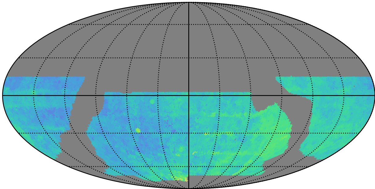
baseline_v2.0_10yrs WFD i band: Median Season Length
