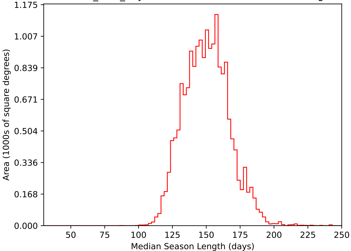
baseline_v2.0_10yrs WFD i band: Median Season Length
