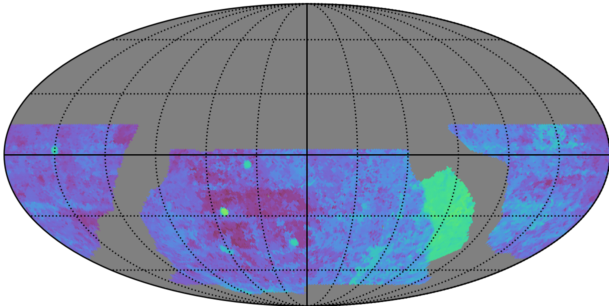
baseline_v2.0_10yrs WFD g band: Median Season Length
