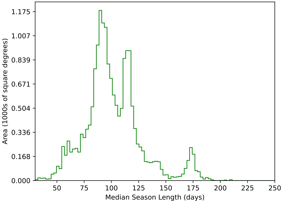
baseline_v2.0_10yrs WFD g band: Median Season Length
