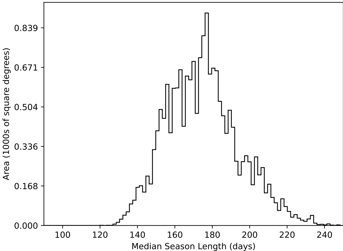
baseline_v2.0_10yrs WFD all bands: Median Season Length
