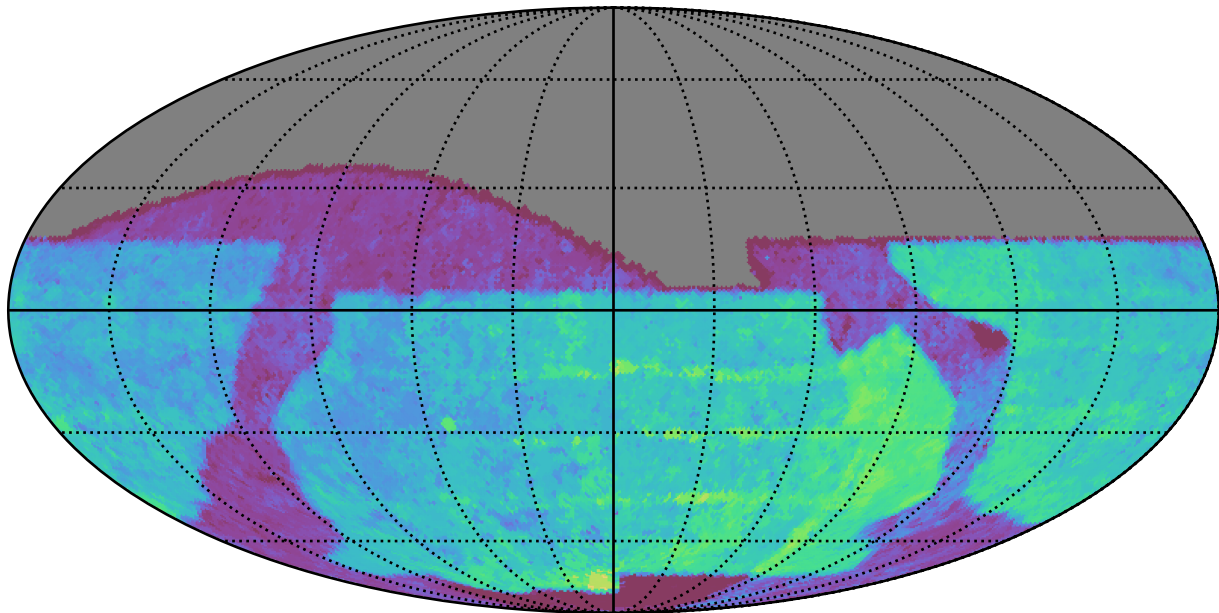
baseline_v2.0_10yrs All sky z band: Median Season Length
