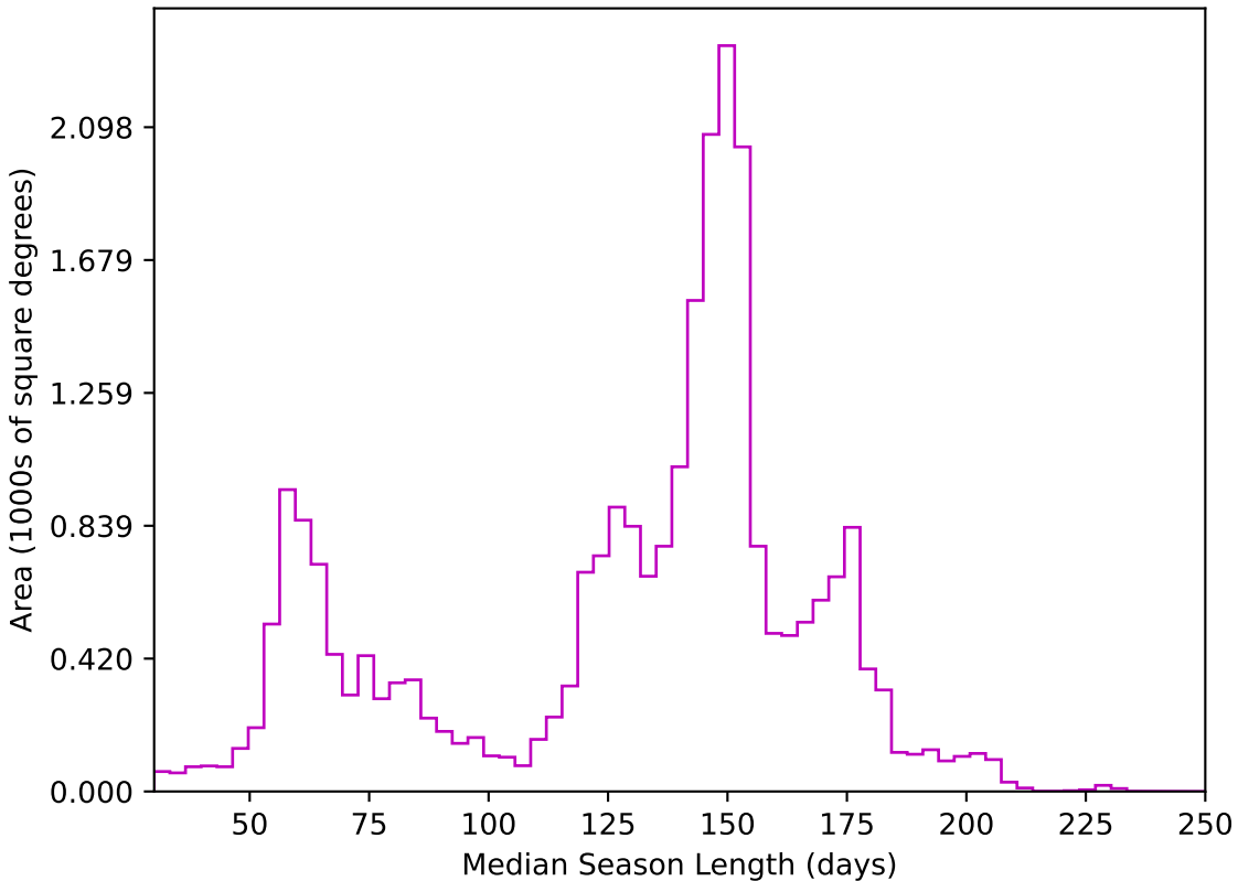
baseline_v2.0_10yrs All sky z band: Median Season Length
