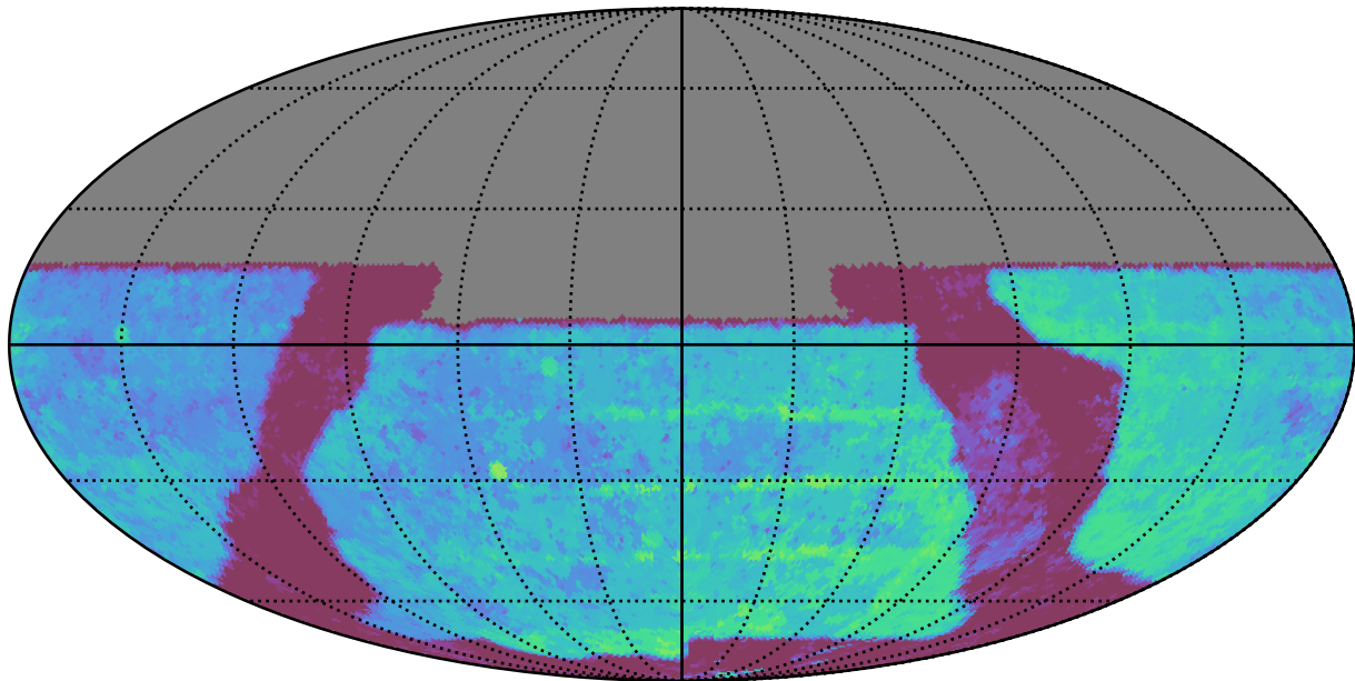
baseline_v2.0_10yrs All sky y band: Median Season Length
