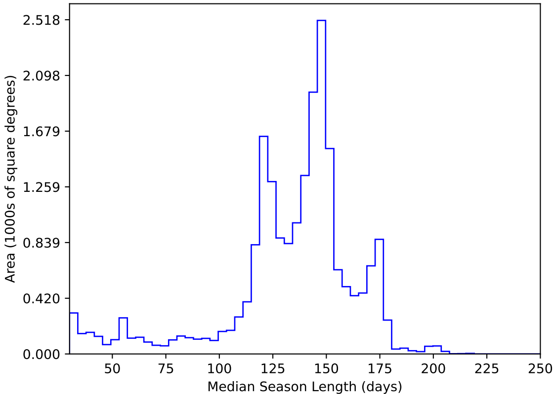
baseline_v2.0_10yrs All sky y band: Median Season Length
