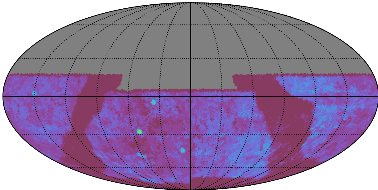
baseline_v2.0_10yrs All sky u band: Median Season Length
