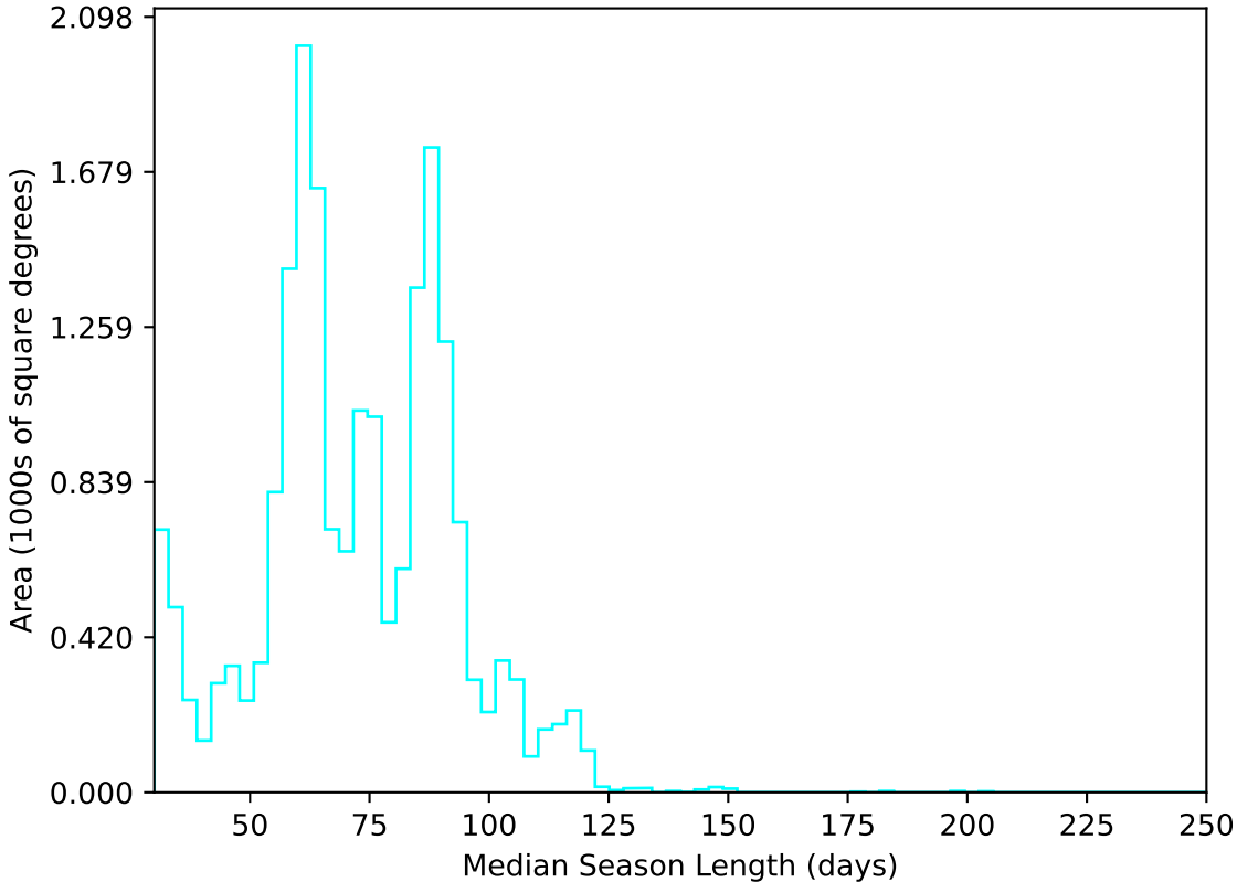
baseline_v2.0_10yrs All sky u band: Median Season Length
