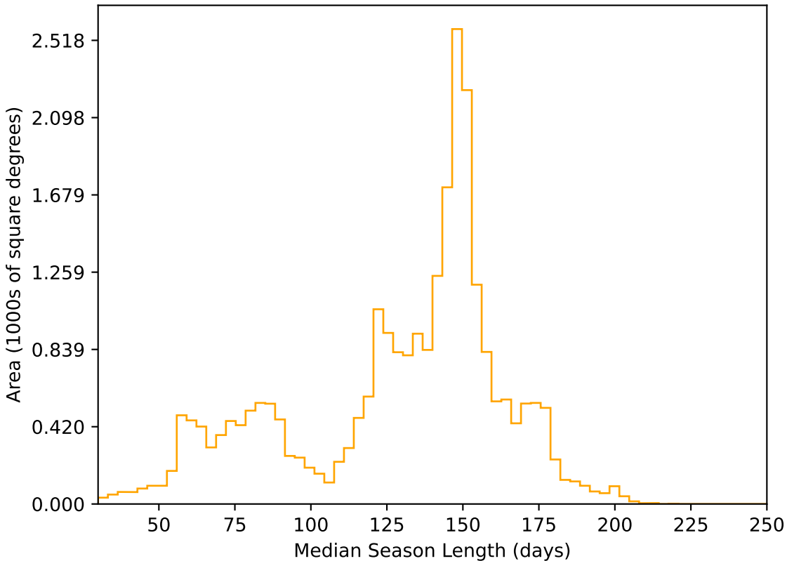
baseline_v2.0_10yrs All sky r band: Median Season Length
