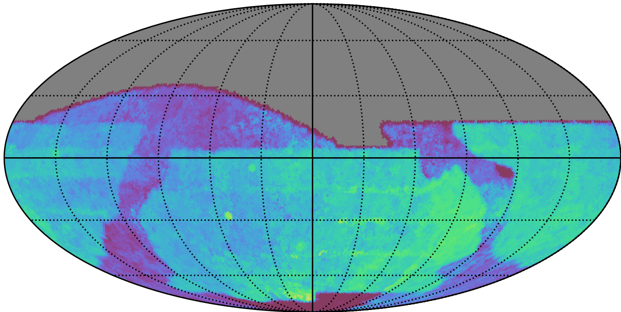
baseline_v2.0_10yrs All sky i band: Median Season Length
