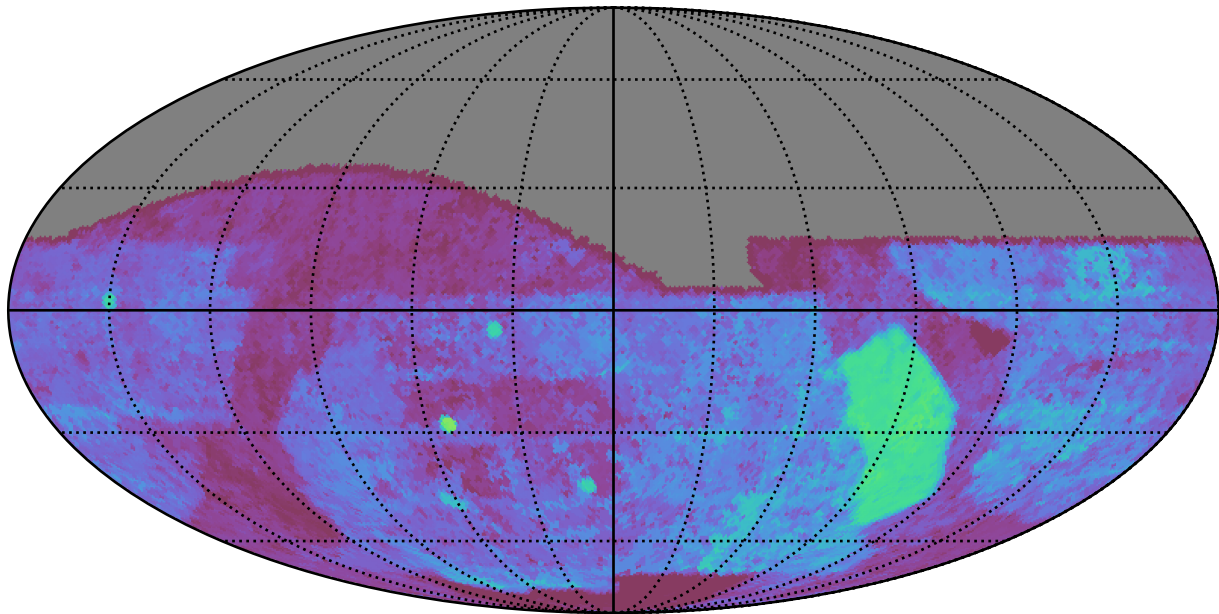
baseline_v2.0_10yrs All sky g band: Median Season Length
