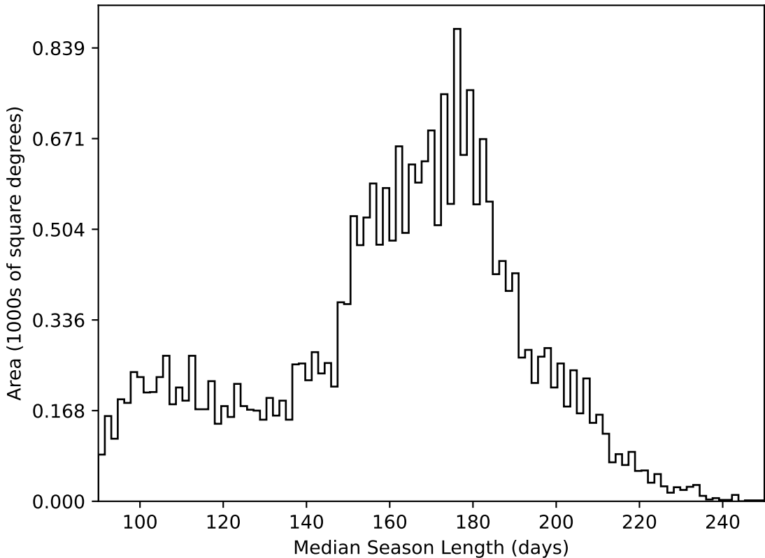
baseline_v2.0_10yrs All sky all bands: Median Season Length
