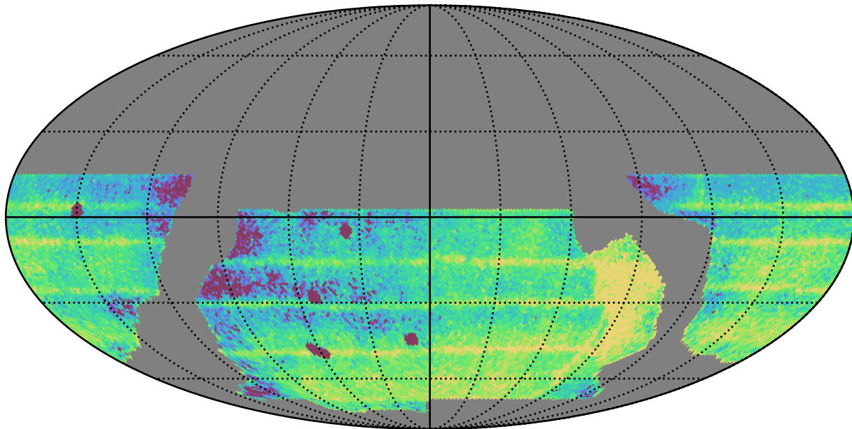
baseline_v2.0_10yrs WFD: Median Intra-Night Gap
