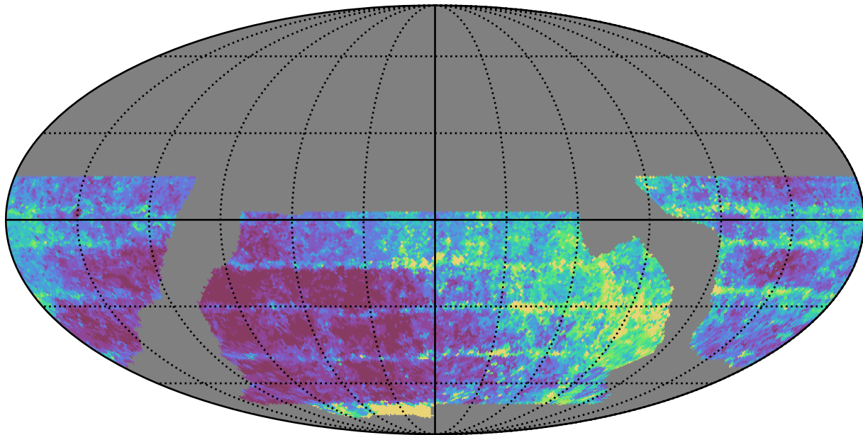
baseline_v2.0_10yrs WFD z band: Median Inter-Night Gap
