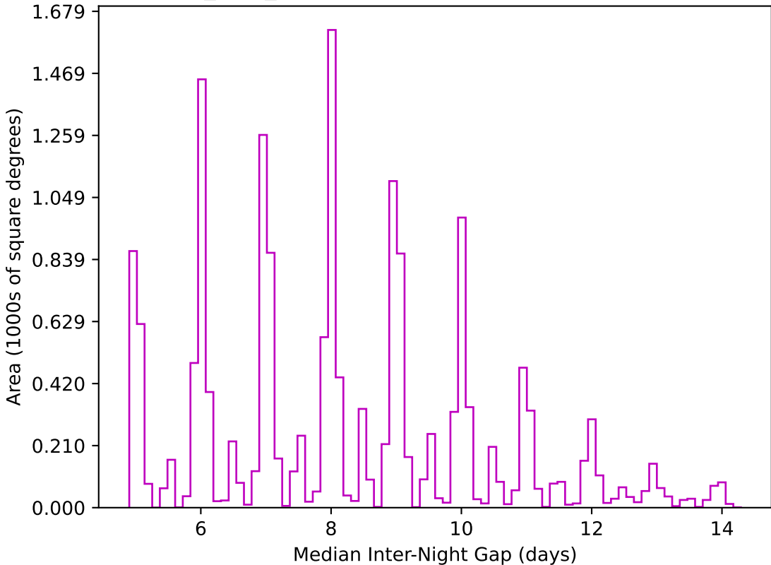
baseline_v2.0_10yrs WFD z band: Median Inter-Night Gap
