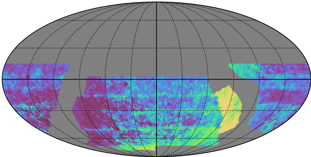
baseline_v2.0_10yrs WFD y band: Median Inter-Night Gap
