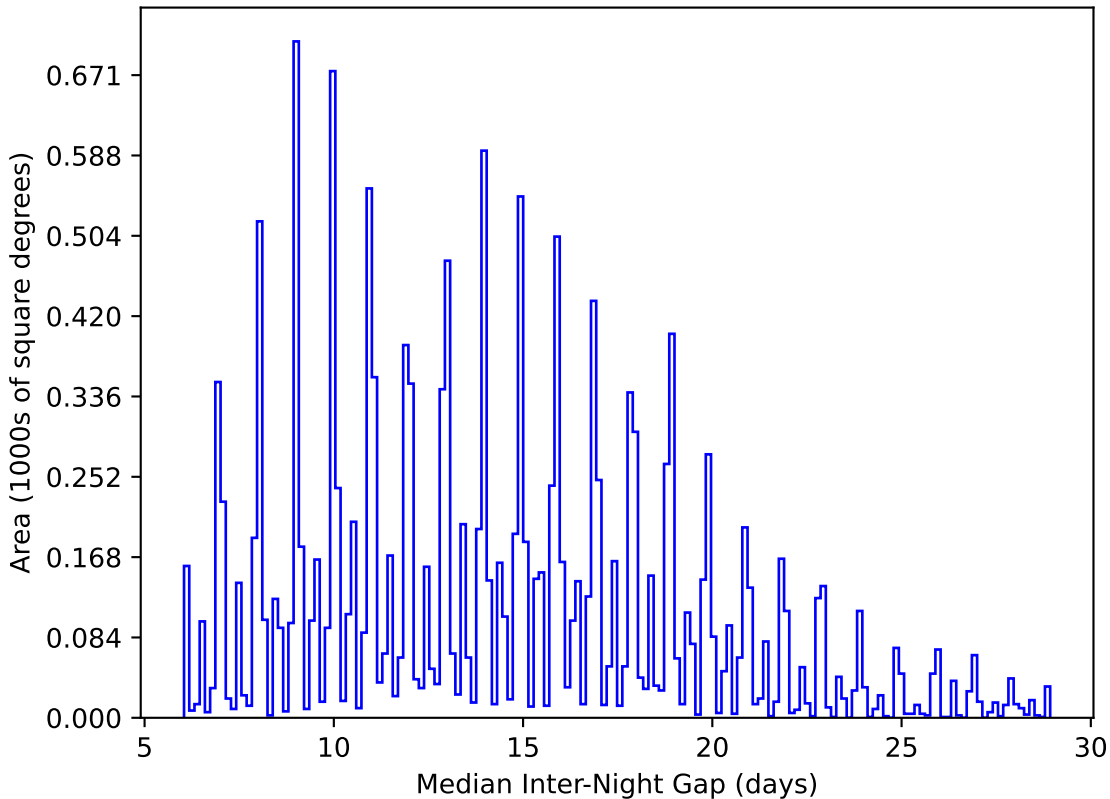
baseline_v2.0_10yrs WFD y band: Median Inter-Night Gap
