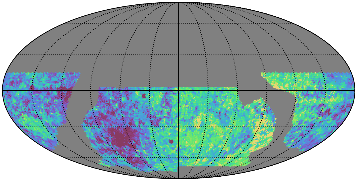
baseline_v2.0_10yrs WFD u band: Median Inter-Night Gap
