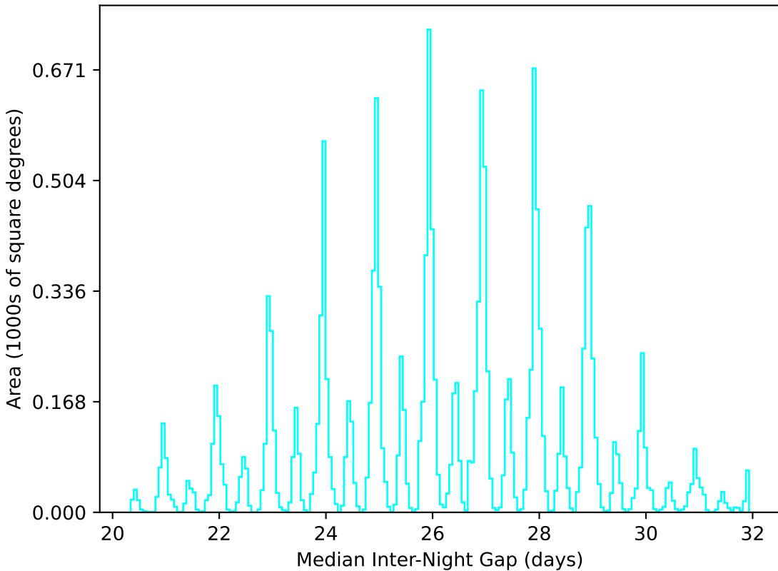
baseline_v2.0_10yrs WFD u band: Median Inter-Night Gap
