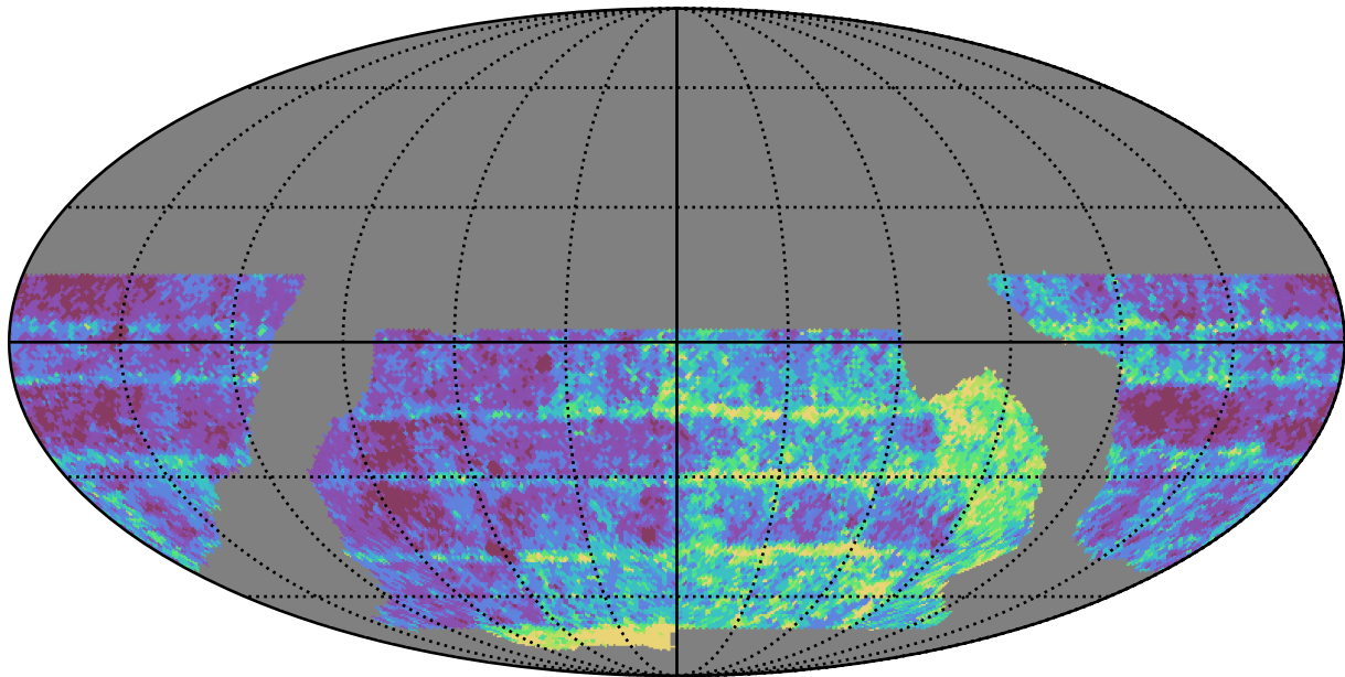
baseline_v2.0_10yrs WFD r band: Median Inter-Night Gap
