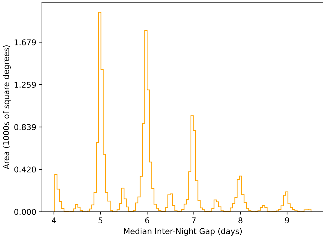
baseline_v2.0_10yrs WFD r band: Median Inter-Night Gap
