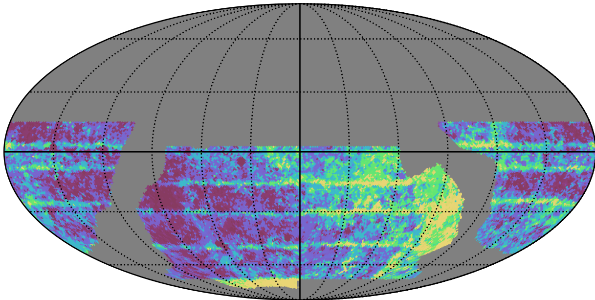
baseline_v2.0_10yrs WFD i band: Median Inter-Night Gap
